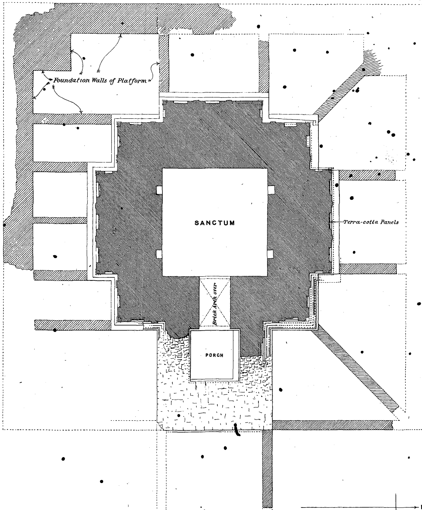
GROUND PLAN.
