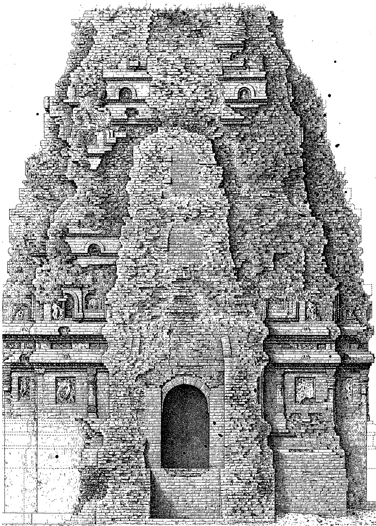
FRONT ELEVATION.
