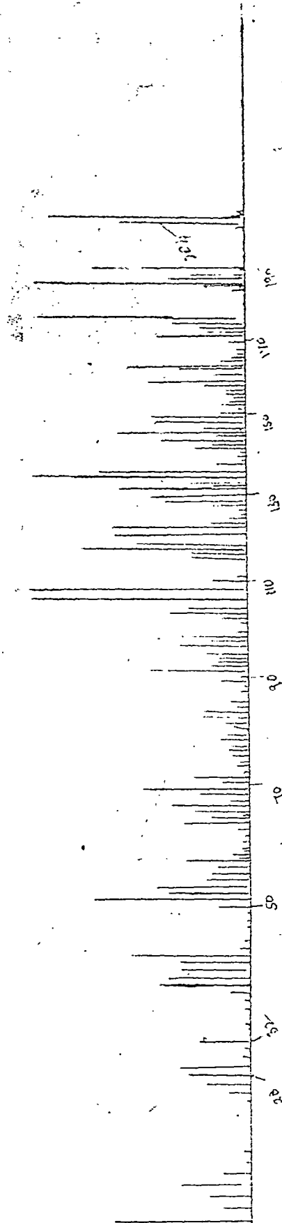
Spectrum 35
