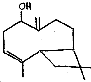
\alpha -Butulenol
