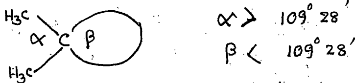
Fig. 9. Suggested bond angles in gem-dimethyl substituted cycloalkanes (Thorpe and Ingold) 55
