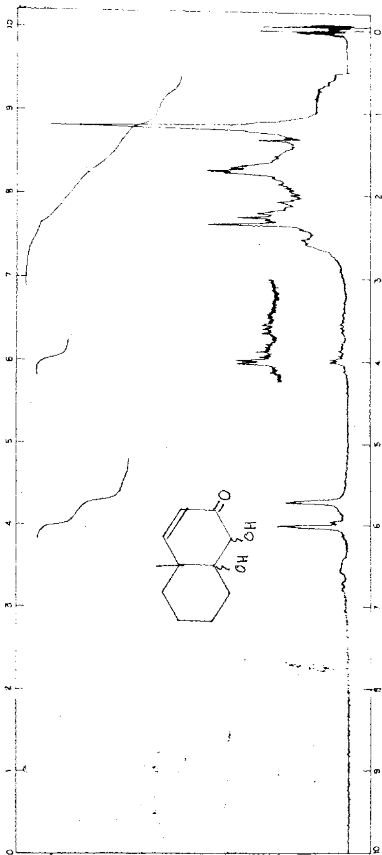
Spectrum 9
