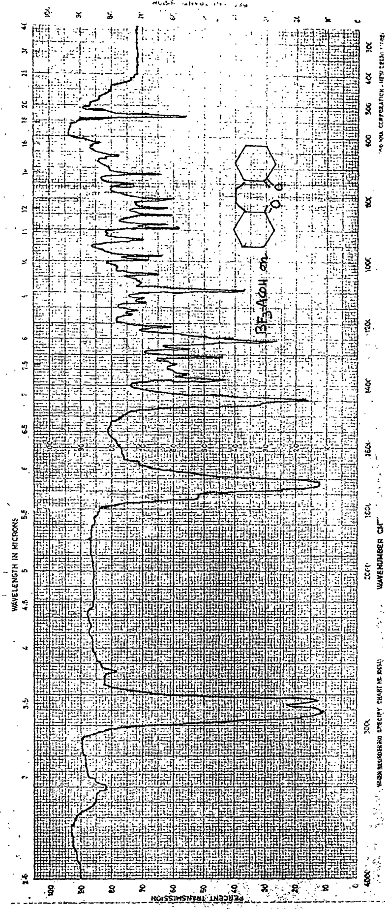
Spectrum 33
