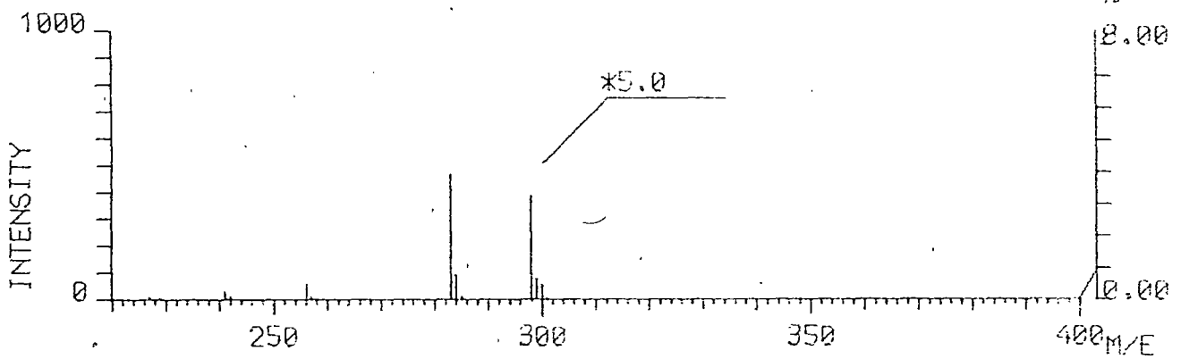
Spectrum 40
