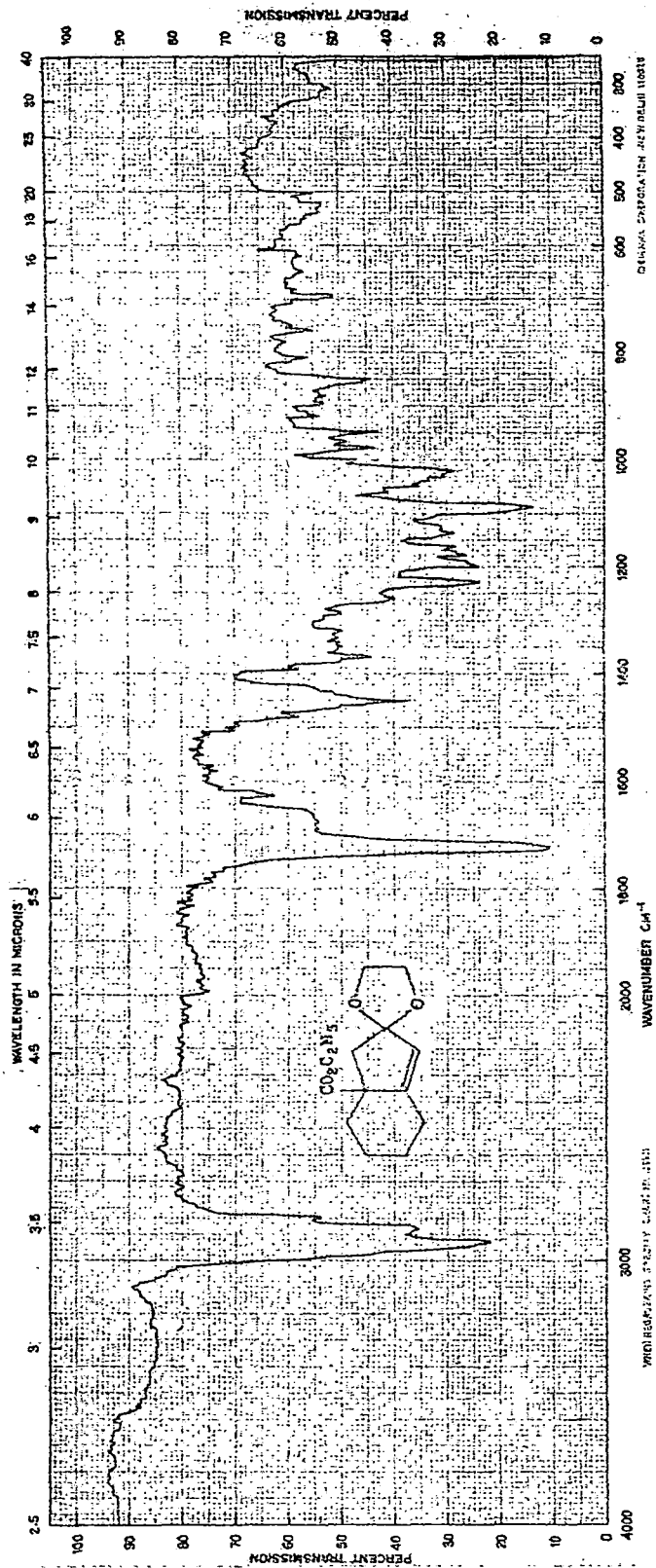
SPECTRUM 13
