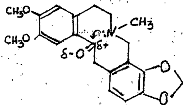
Cryptopine
