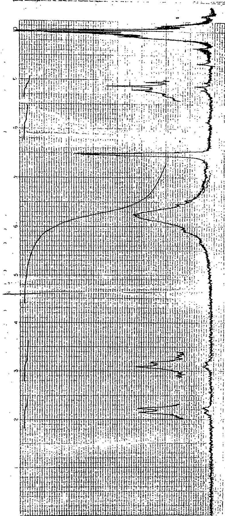
SPECTRUM 45
