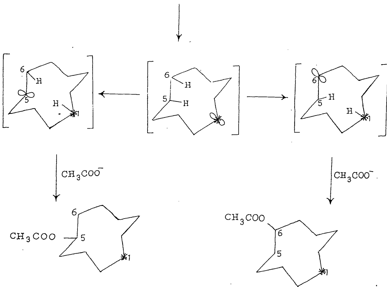
Acetolysis of cyclodecyl tosylate.
