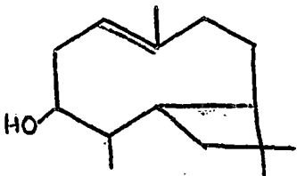
\beta - Butulenol
