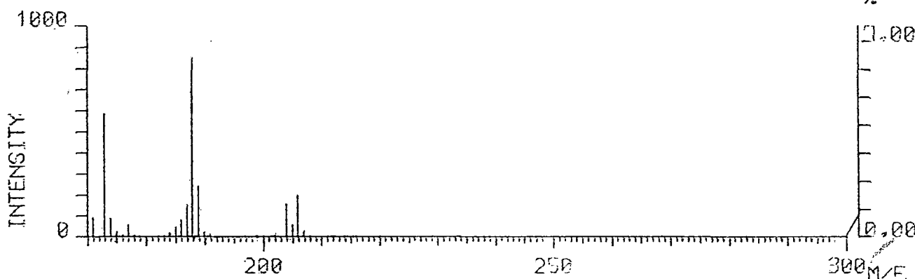
Spectrum 52
