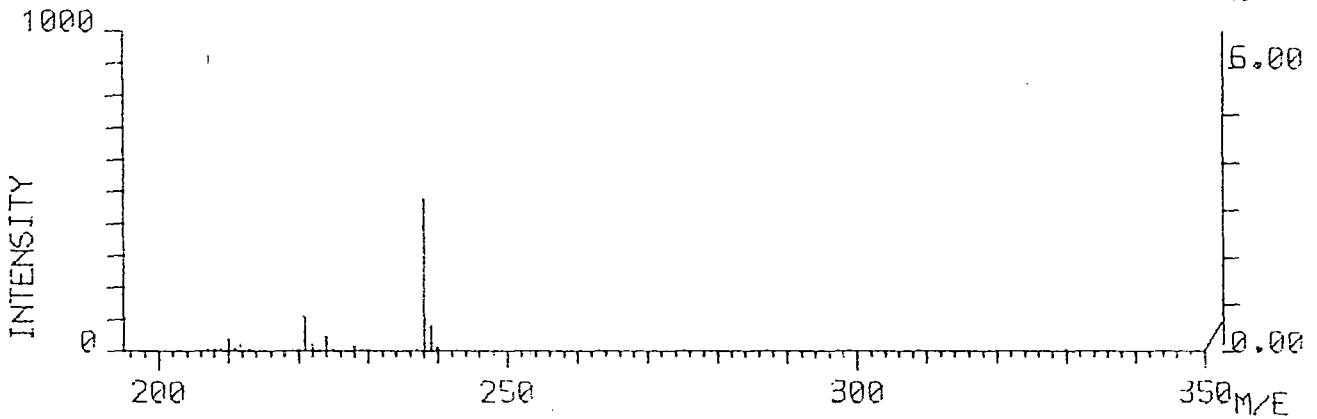
SPECTRUM 46
