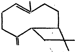
Caryophyllene
