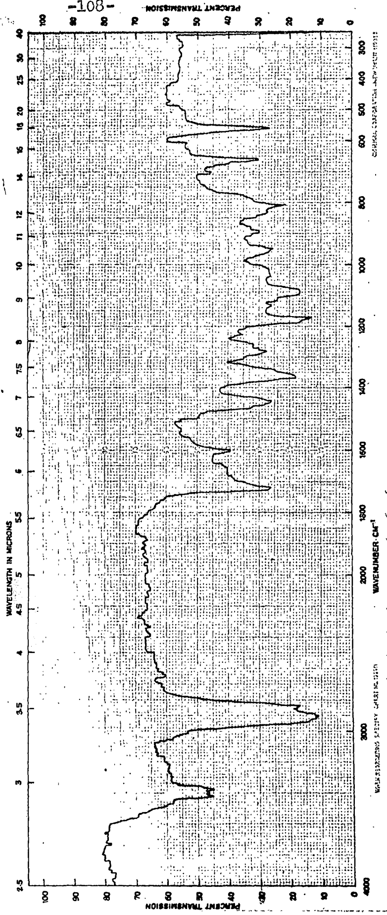
Spectrum 18
