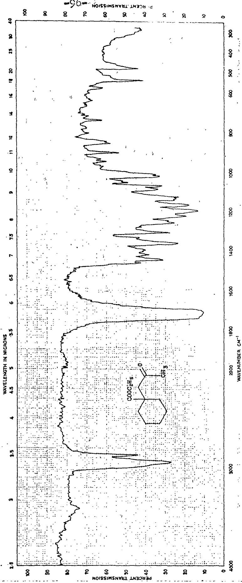
S PECTRUM 11
