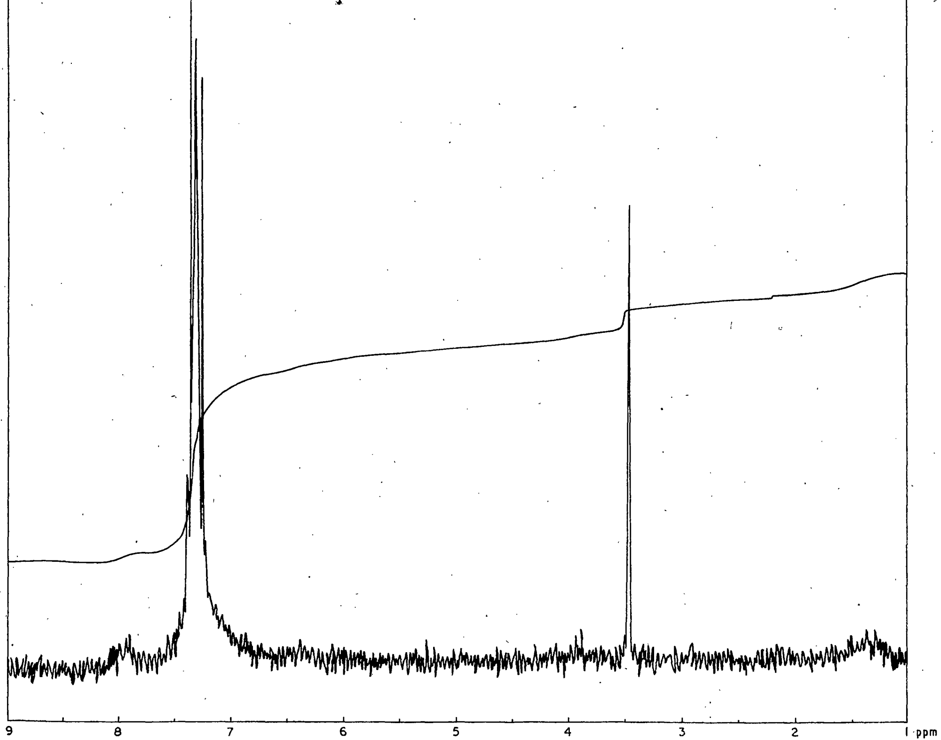
FIG. 16C: PMR SPECTRUM OF PHENYLTIN CHLORIDE METHOXY N - PHENYLBENZOHYDROXAMATE IN \text{CDCl}_3 ( 60 MHz )
