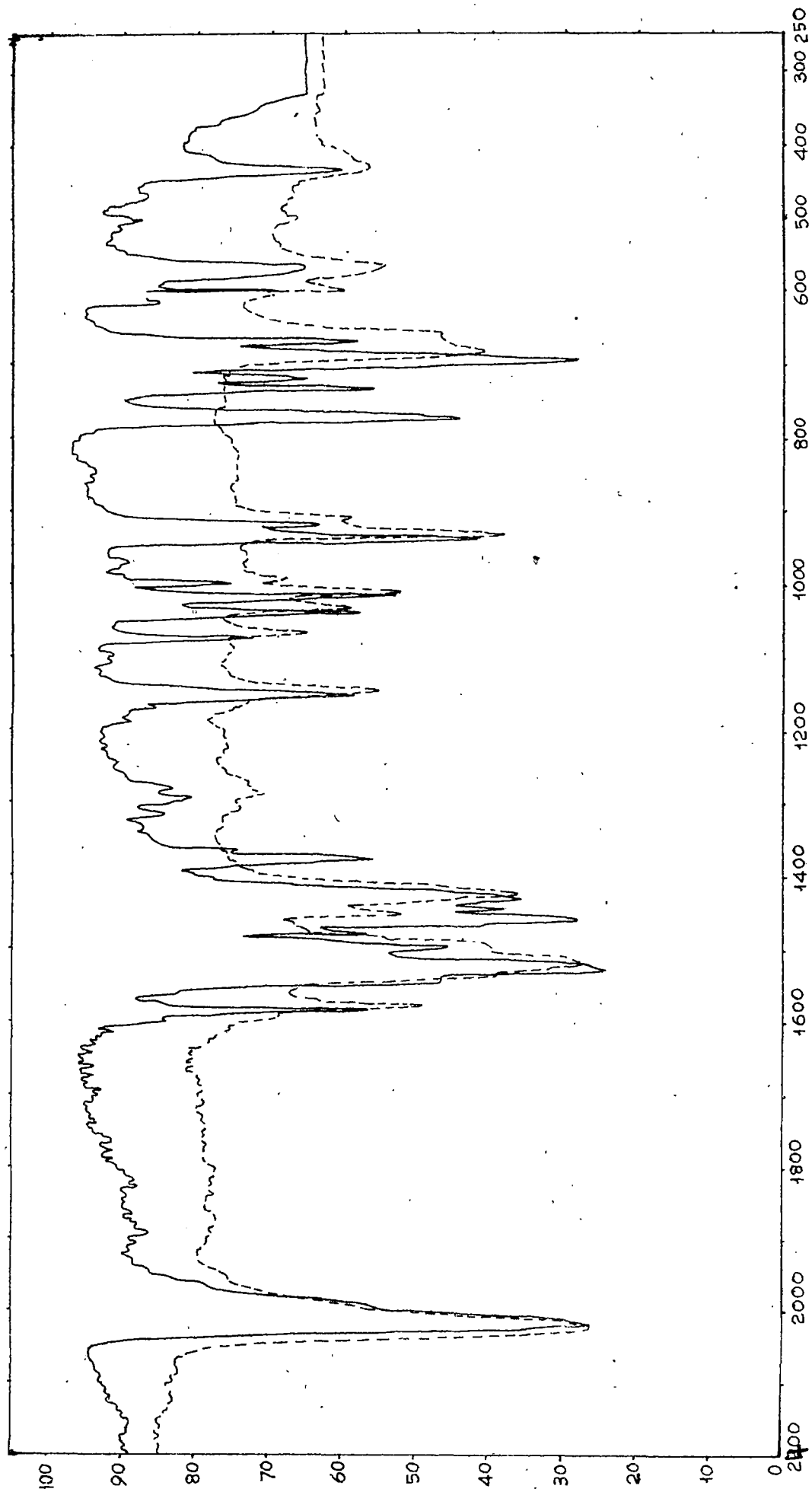
Fig:- 8e. IR Spectrum of Phenyltin thiocyanate bis( N-Phenylbenzohydroxamate )
