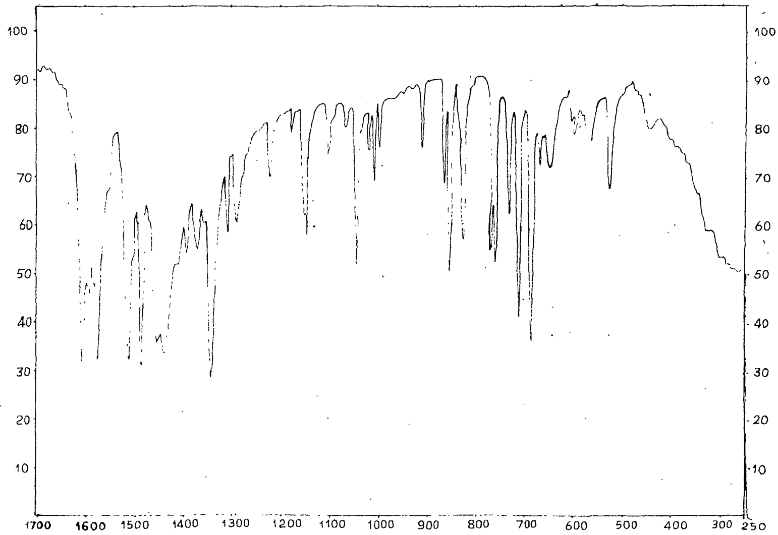
I.R. Spectrum of N-Phenylparanitrobenzohydroxamic Acid .
