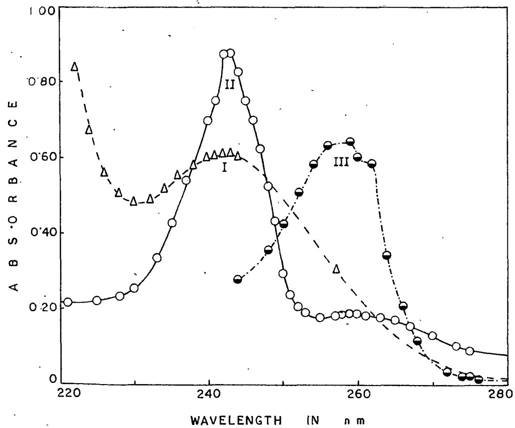
FIG. 18b TETRAPHENYLDITIN DIACETATE IN CYCLOHEXANE (I) DIOXINATE DITIN DIACETATE IN CYCLOHEXANE (II) AND IN CHLOROFORM (III).
