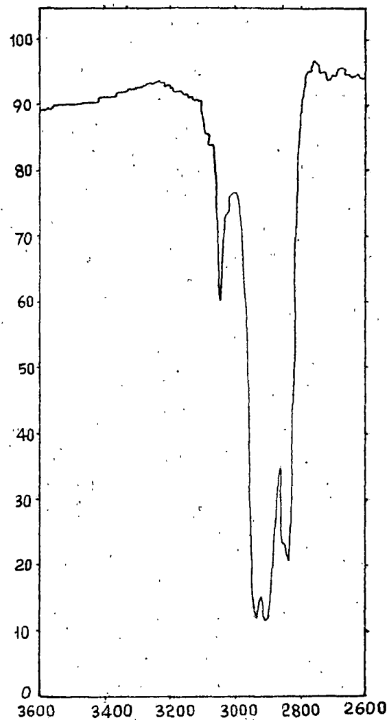
I.R. Spectrum of Dibutyltin bis(N-Phenylbenzohydroxamate)
