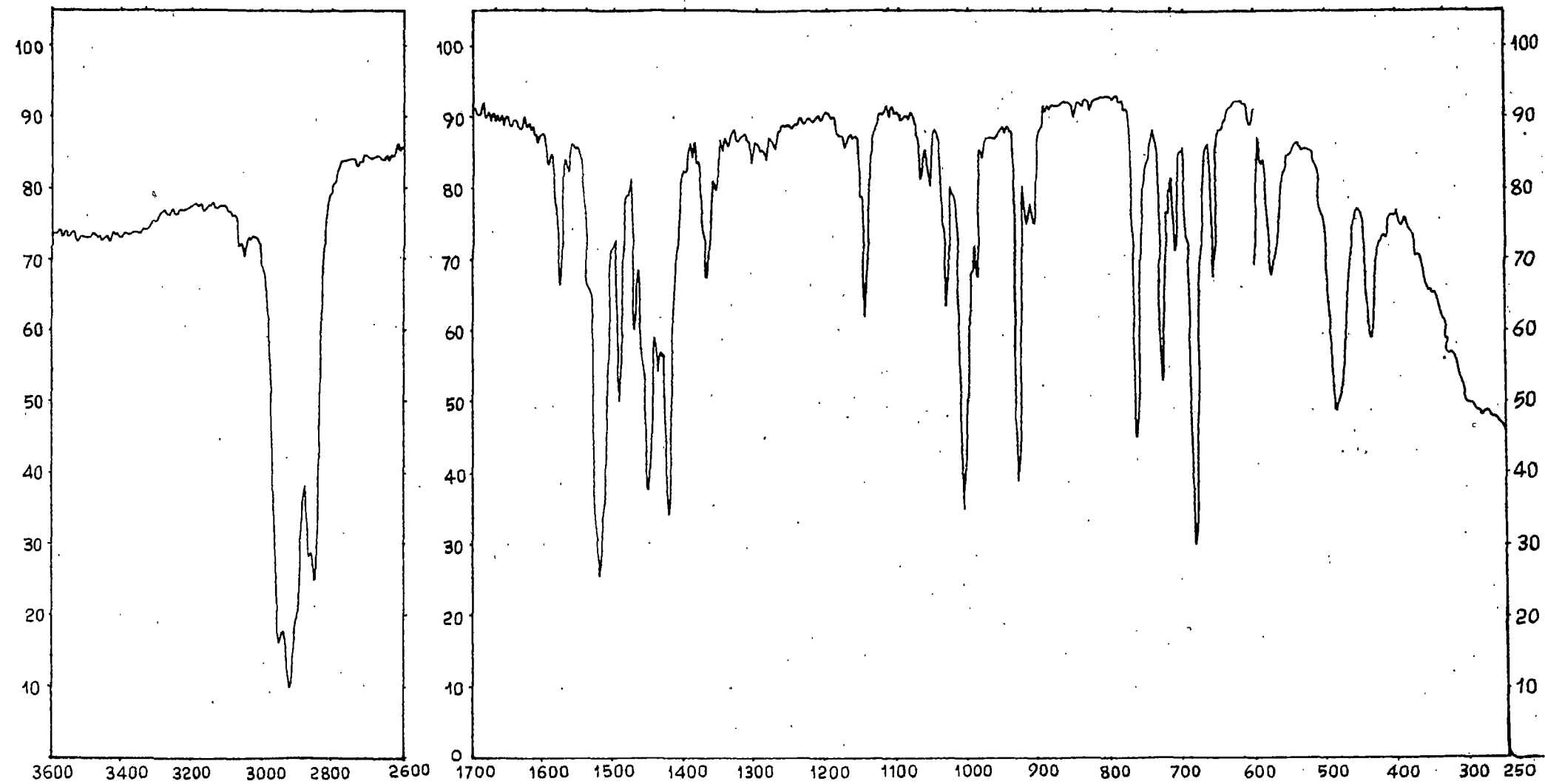
I.R. Spectrum of Phenylbromotin methoxy N-Phenylbenzohydroxamate
