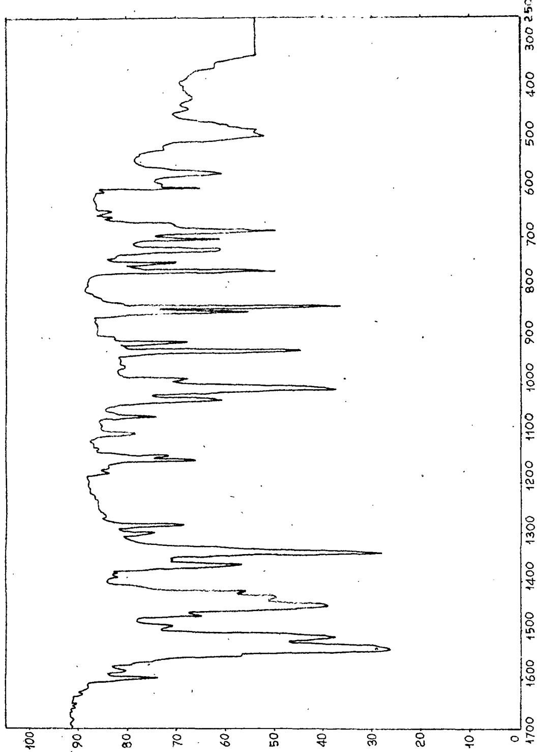
I.R Spectrum of Phenyllin Chloride methoxy N-Phenylparanitrobenzohydroxamate
