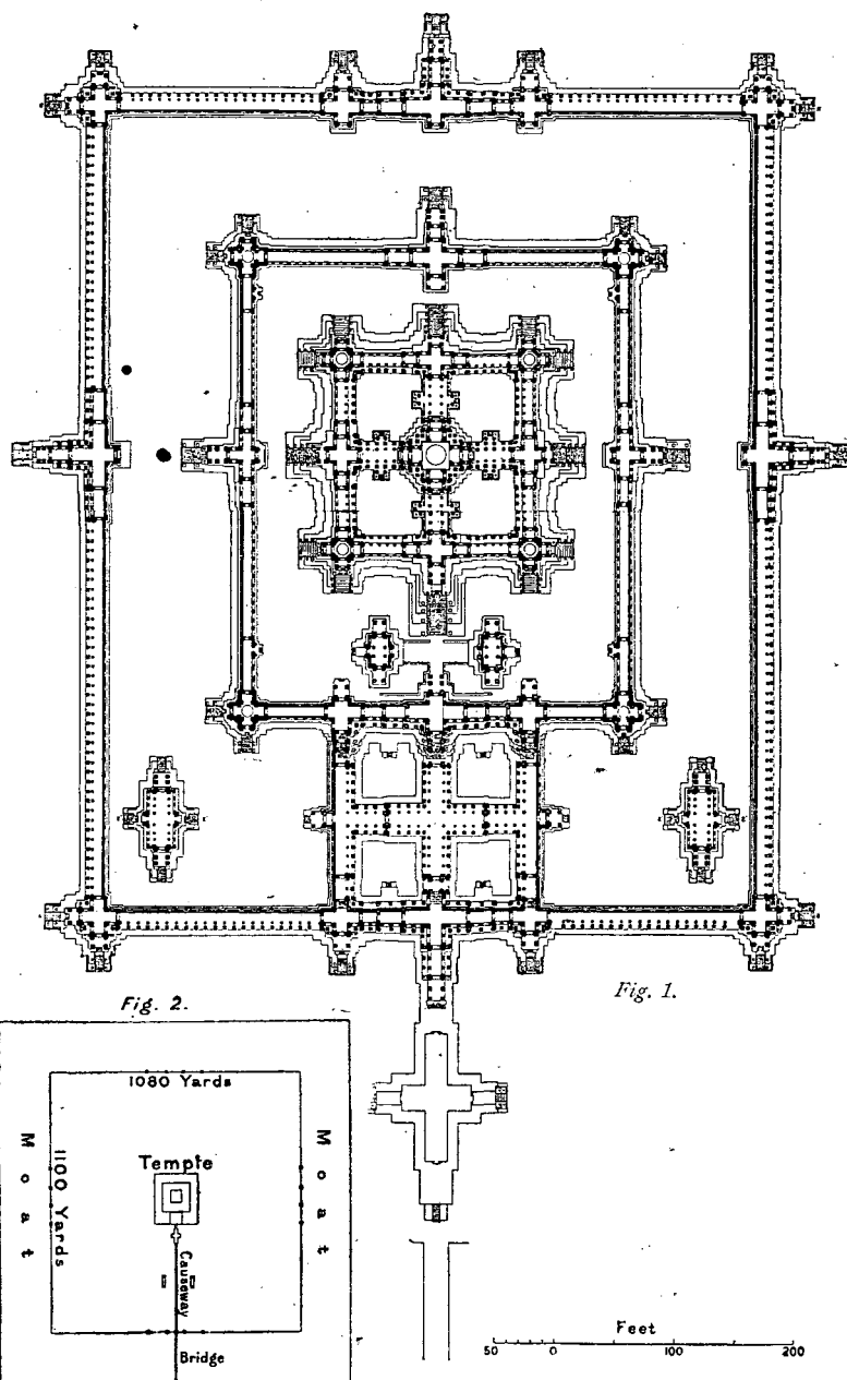
459. Plan of the temple of Angkor Vât. Scale 176\frac{1}{2} ft. to 1 in.
