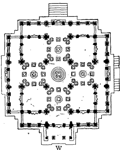
279. Plan of Nandisvara-dvîpa Temple at Satrunjaya. Scale 25 ft. to 1 in.
