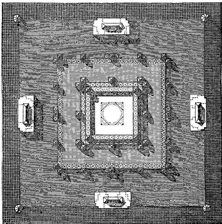
Plan of Akbar's Tomb at Sikandara. (From a Plan by the Author.) Scale 100 ft. to 1 in.
