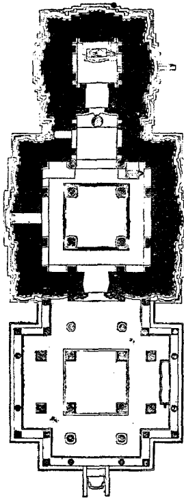
276. Lakkundi Jaina Temple. Scale 25 ft. to 1 in. (From Plan by Mr H. Cousens.)
