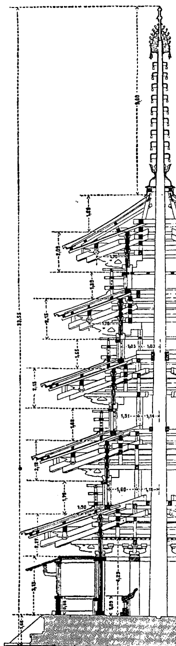
512. Section of the Hôriuji Pagoda. From Baltzer.
