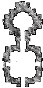
317. Plan of Rājārānī Temple. (Compiled from a Plan by Bābu Rājendralāl and corrected from Photographs.) Scale 50 ft. to 1 in.
