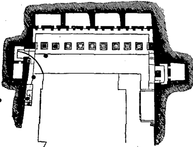
268. Upper storey, Rānī-gumpha. Scale 50 ft. to 1 in.
