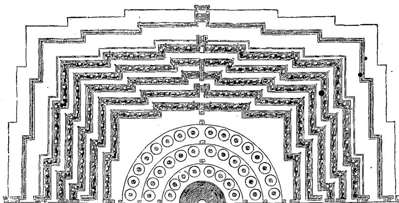
477. Half-plan of Temple of Boro-Budur. (From a Plate in the second edition of Sir Stamford Raffles' 'History of Java.') Scale 100 ft. to 1 in.
