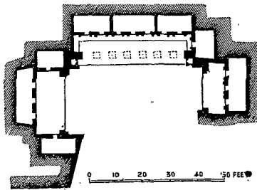
269. Lower storey, Rānī-gumpha. (From Plans by H. H. Locke.)
