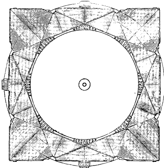
416. Pendentives of the Tomb of Muhammad, looking upwards. (From a Drawing by Mr Cumming.) Scale 50 ft. to 1 in.
