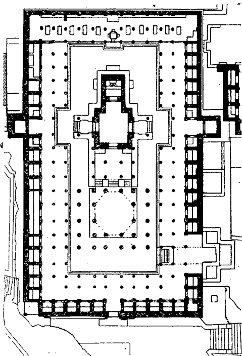
285. Temple of Tejahpála, Mount Ábú. (From a Plan by Mr. H. Cousens.) Scale 50 ft. to 1 in.
