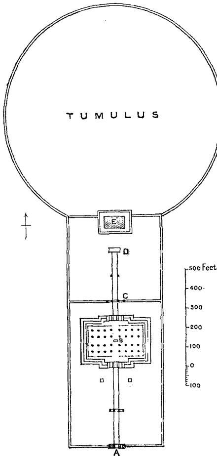
497. Plan of the Tomb of Yung-lo.
