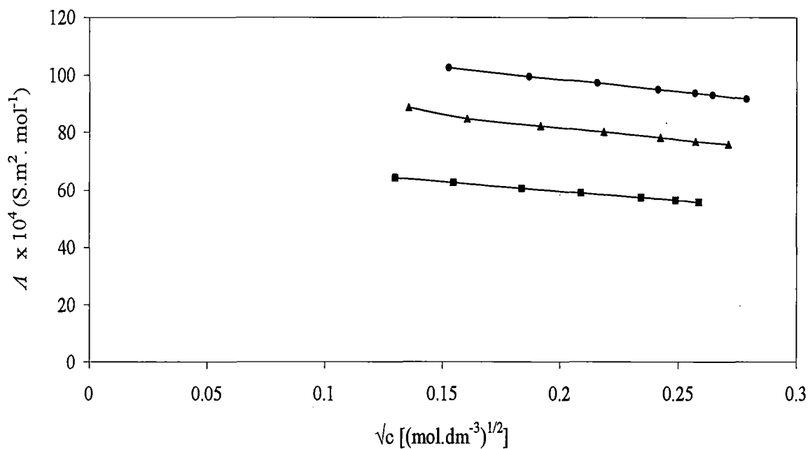
Fig.2. The plots of equivalent conductances A versus \sqrt{c} for KBr in different mass% of glycerol in mixtures at 298.15 K. Experimental points: 10% (●), 20% (▲), 30% (■).
