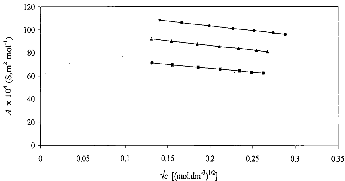
Fig.3. The plots of equivalent conductances A versus \sqrt{c} for KI in different mass% of glycerol in mixtures at 298.15 K. Experimental points: 10% (●), 20% (▲), 30% (■).
