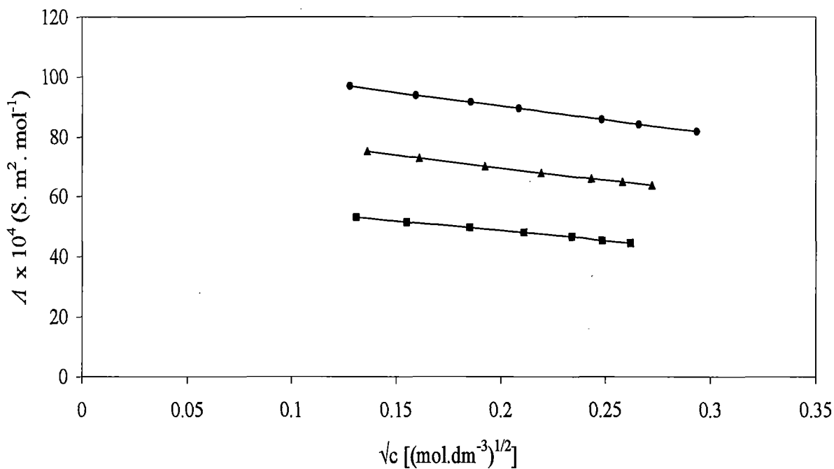
Fig.1. The plots of equivalent conductances A versus \sqrt{c} for KCl in different mass% of glycerol in mixtures at 298.15 K. Experimental points: 10% (●), 20% (▲), 30% (■).
