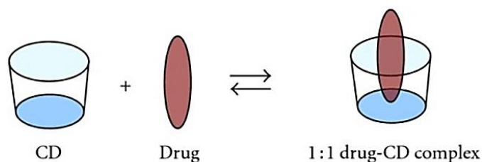
Scheme 1 Diagrammatic representation of the probable complexes obtained
