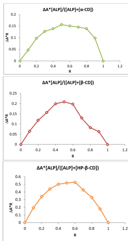
Fig. 2 Job's Plot for [ALP] with a) \alpha -CD, b) \beta -CD and c) HP- \beta -CD
