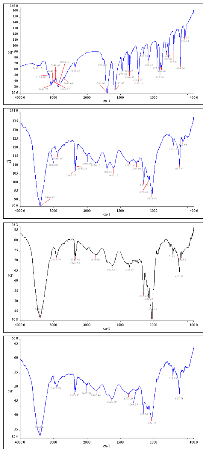
Fig. 7 FT-IR spectra of 1:1 inclusion complexes a) [ALP] + b) [ALP] + \alpha -CD, c) [ALP] + \beta -CD and d) [ALP] + HP- \beta -CD at 298.15K
