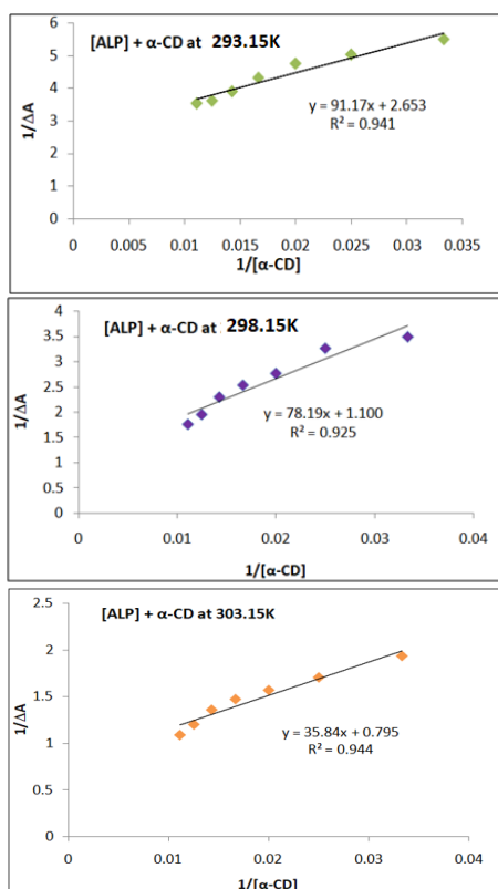
Fig. 3 Benesi-Hildebrand double reciprocal plots for the effect of \alpha -CD on the absorbance of [ALP] at a) 293.15 K, b) 298.15 K and c) 303.15K
