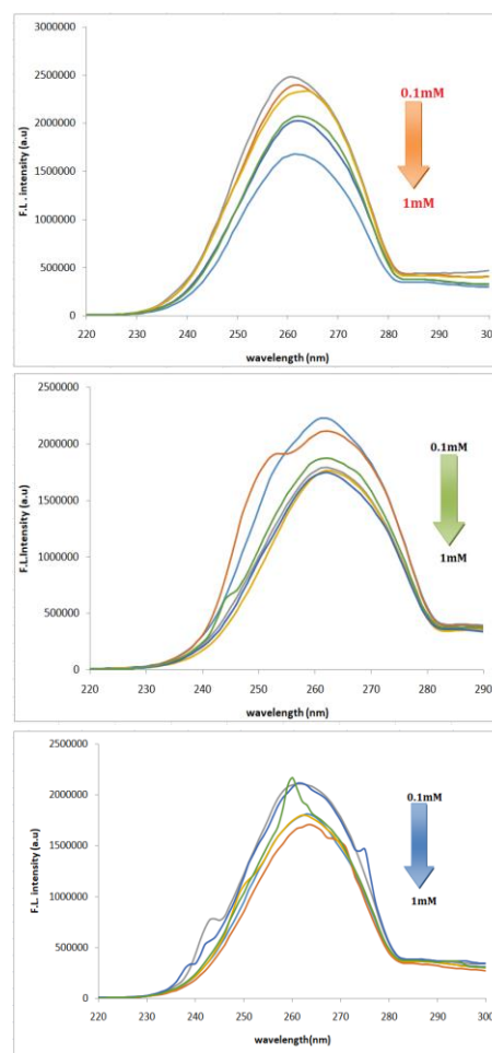
Fig. 6 Fluorescence emission spectrum of aqueous a) \alpha -CD, b) \beta -CD and c) HP- \beta -CD in presence of (0.1mM–1.0 mM) of ALP ( \lambda_{ex} =250 nm, slit width =5/5).
